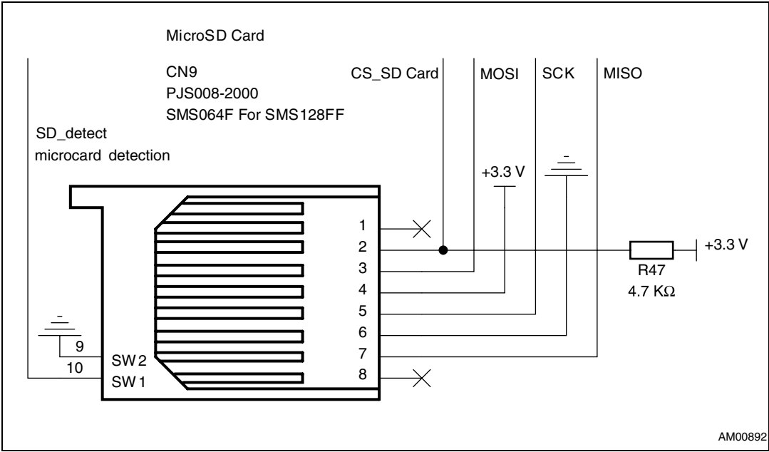
Figure 24. MicroSD Card
