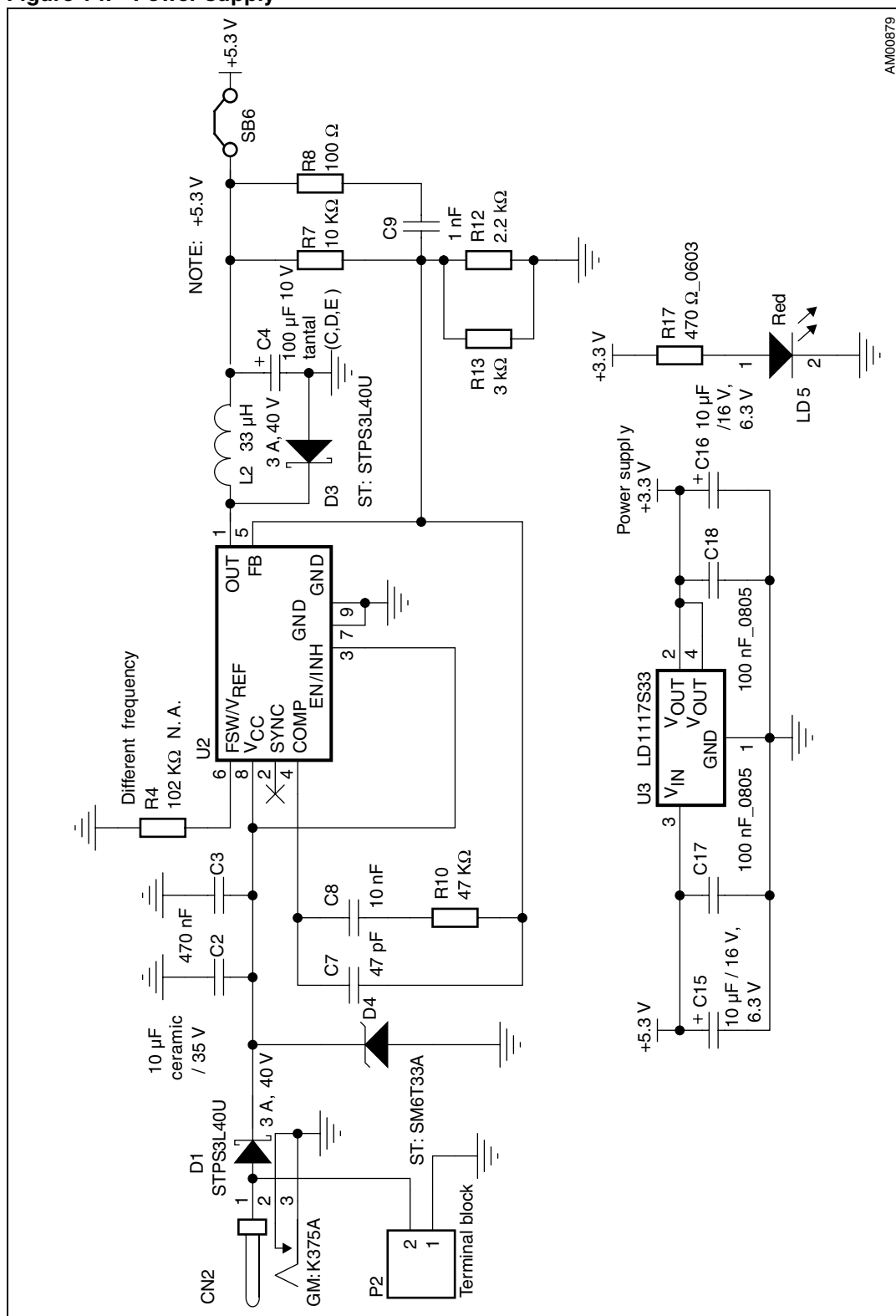
Figure 14. Power supply
